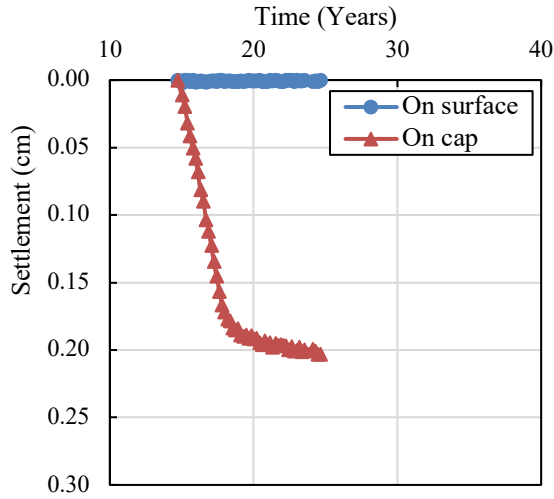
Fig.8 Settlement during third pile load test
