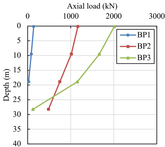
Fig.9 Comparison of axial load of each test
