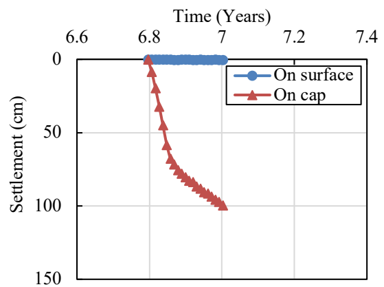
Fig.6 Settlement during first pile load test
