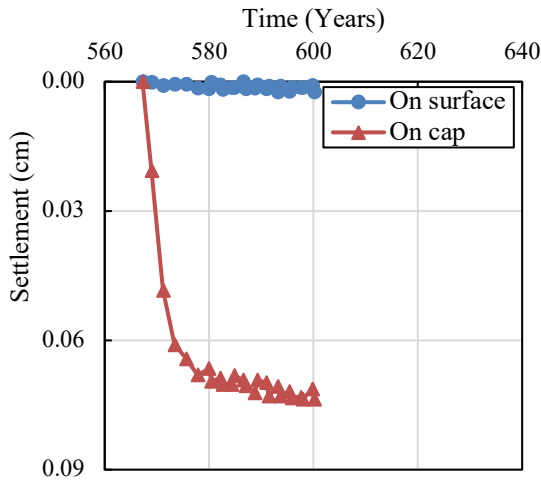
Fig.7 Settlement during second pile load test
